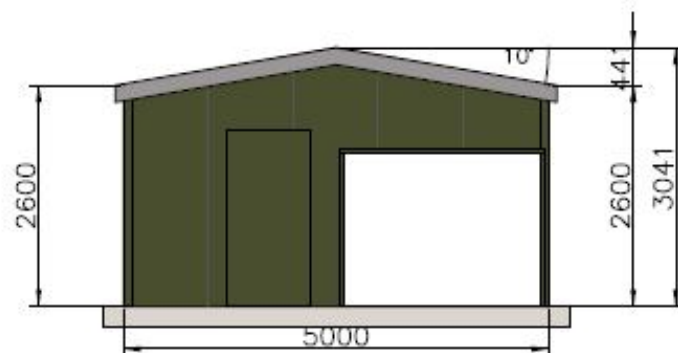
Front Elevation (External)
