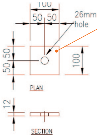
Plate Washer PW2
