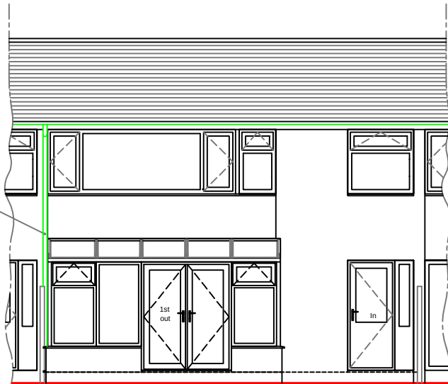
REAR ELEVATION
