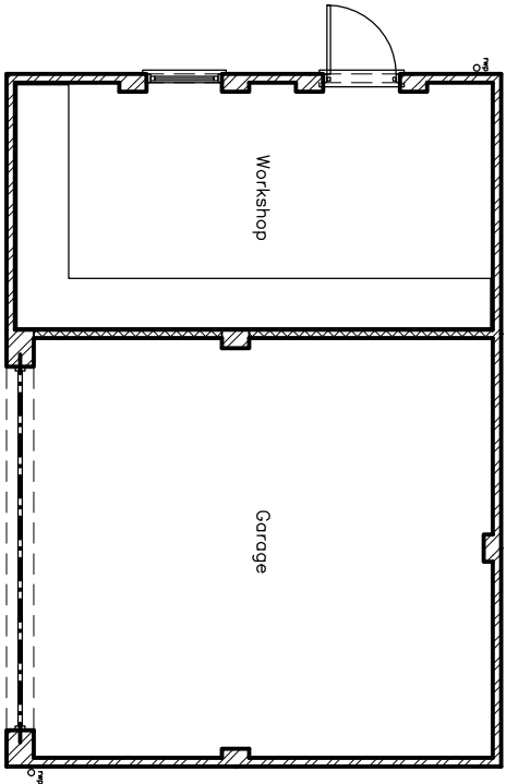
Floor Plan 1:100
