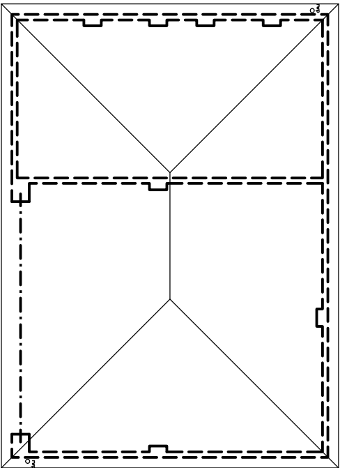
Roof Plan
