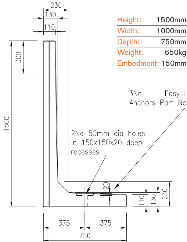
Side Elevation
