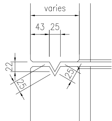
Joint Detail (1:5)
