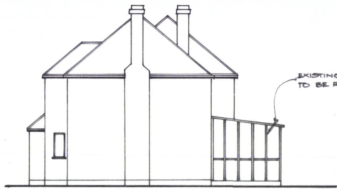
WEST ELEVATION
