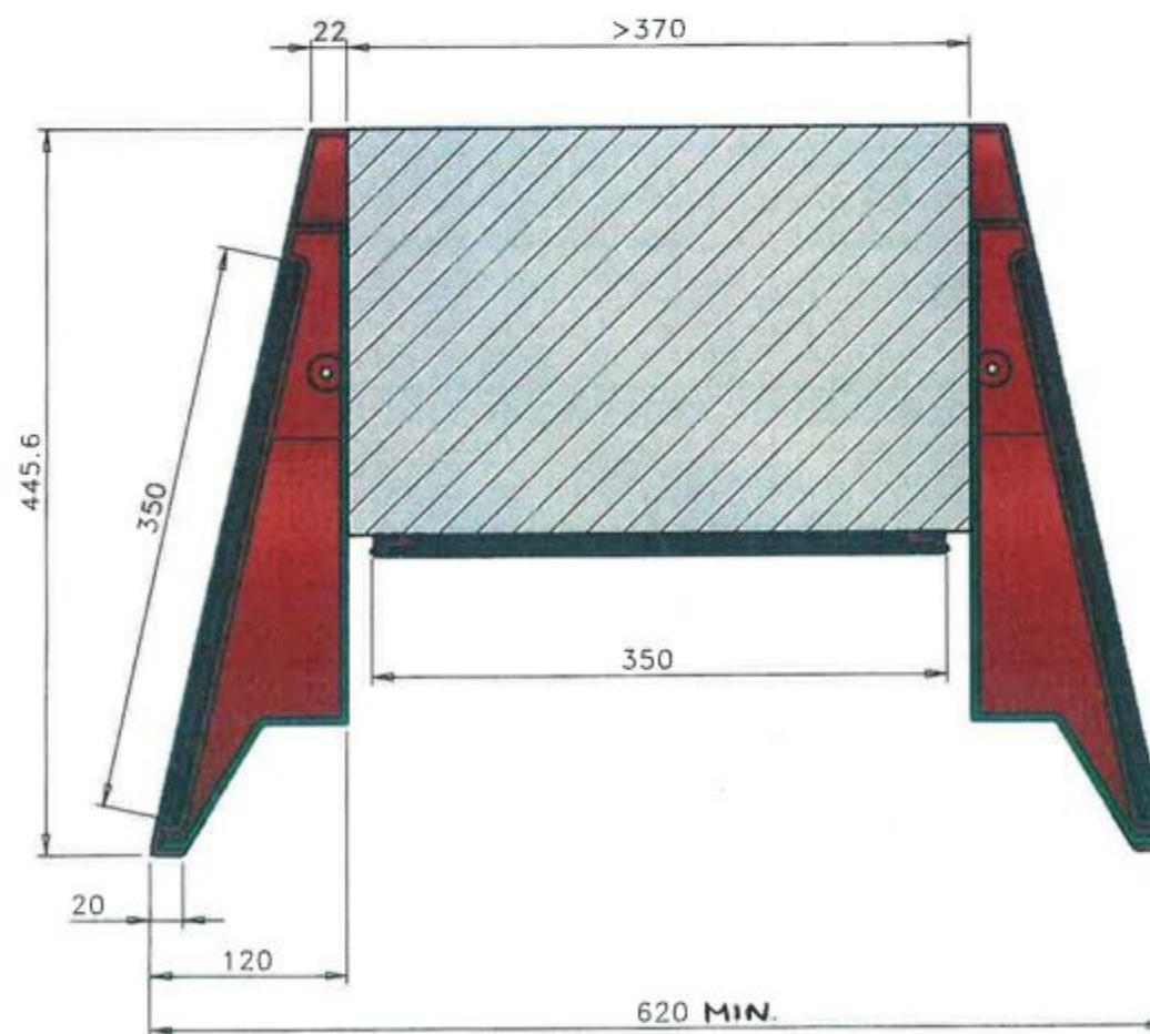
SECTION E-E SCALE 1 : 5
