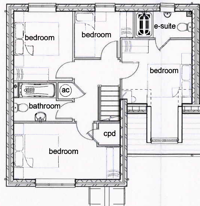
2 First Floor
