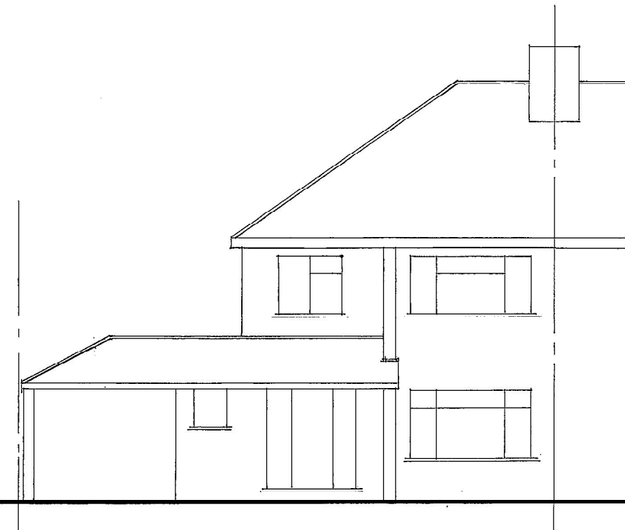
Existing SE/Front Elevation
