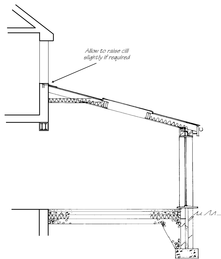
Cross-Section
