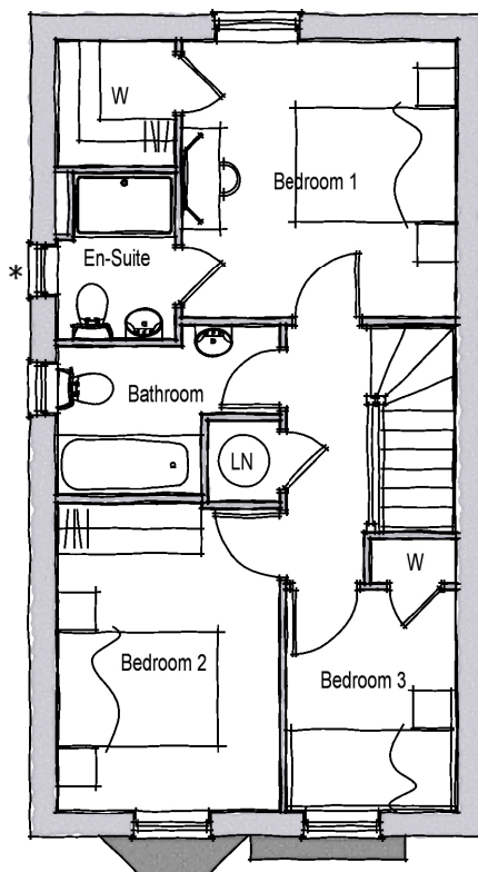
FIRST FLOOR PLAN * WINDOW TO PLOT 67 ONLY.
