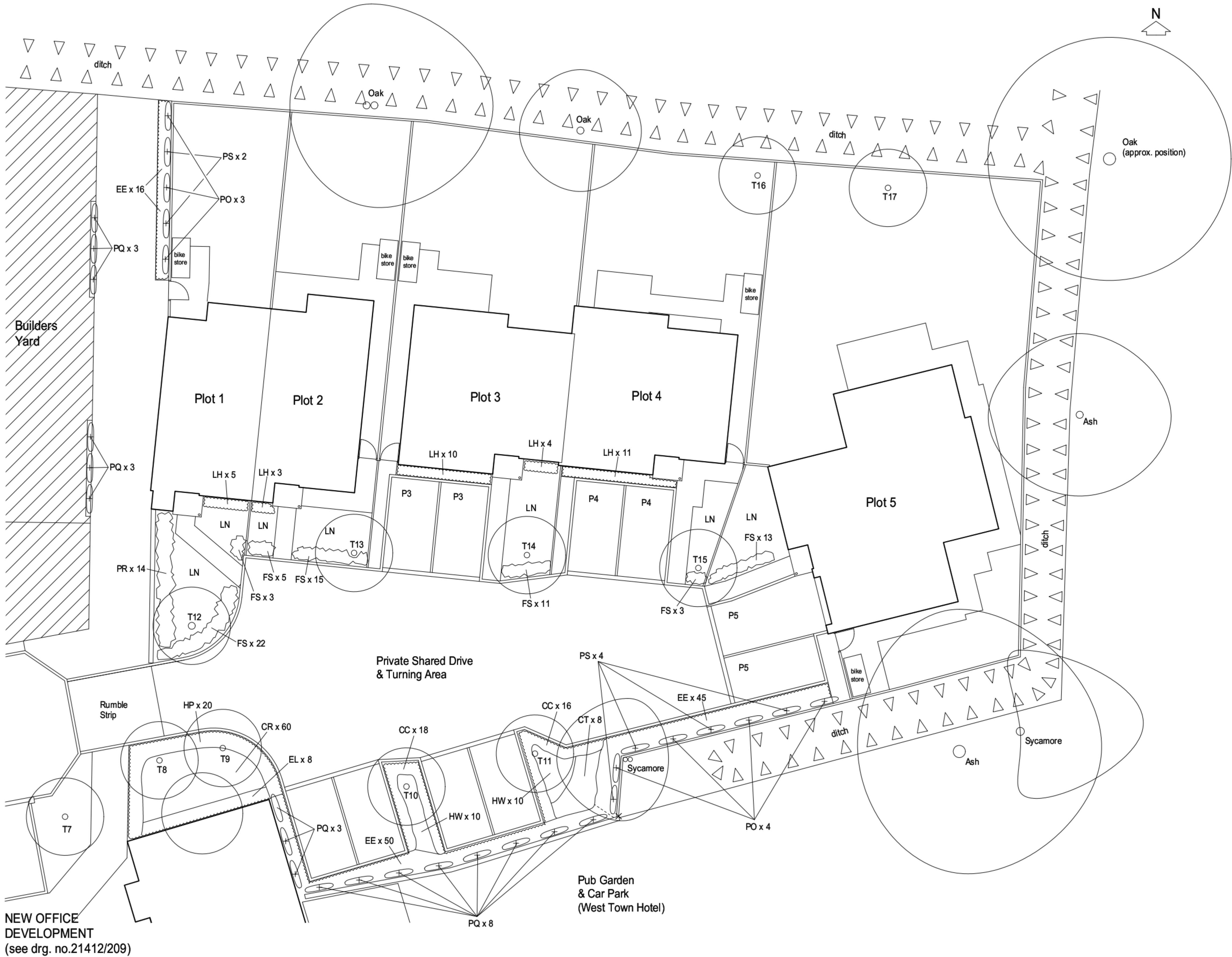
Proposed Soft Landscaping Plan - Residential Site 1:100
