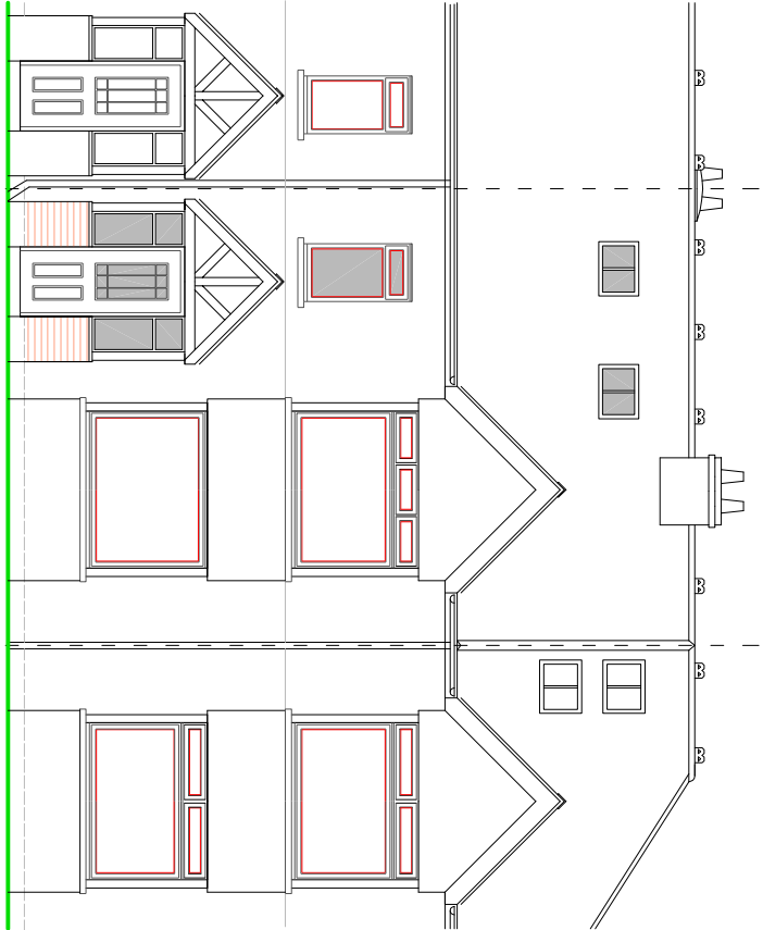
FRONT ELEVATION
