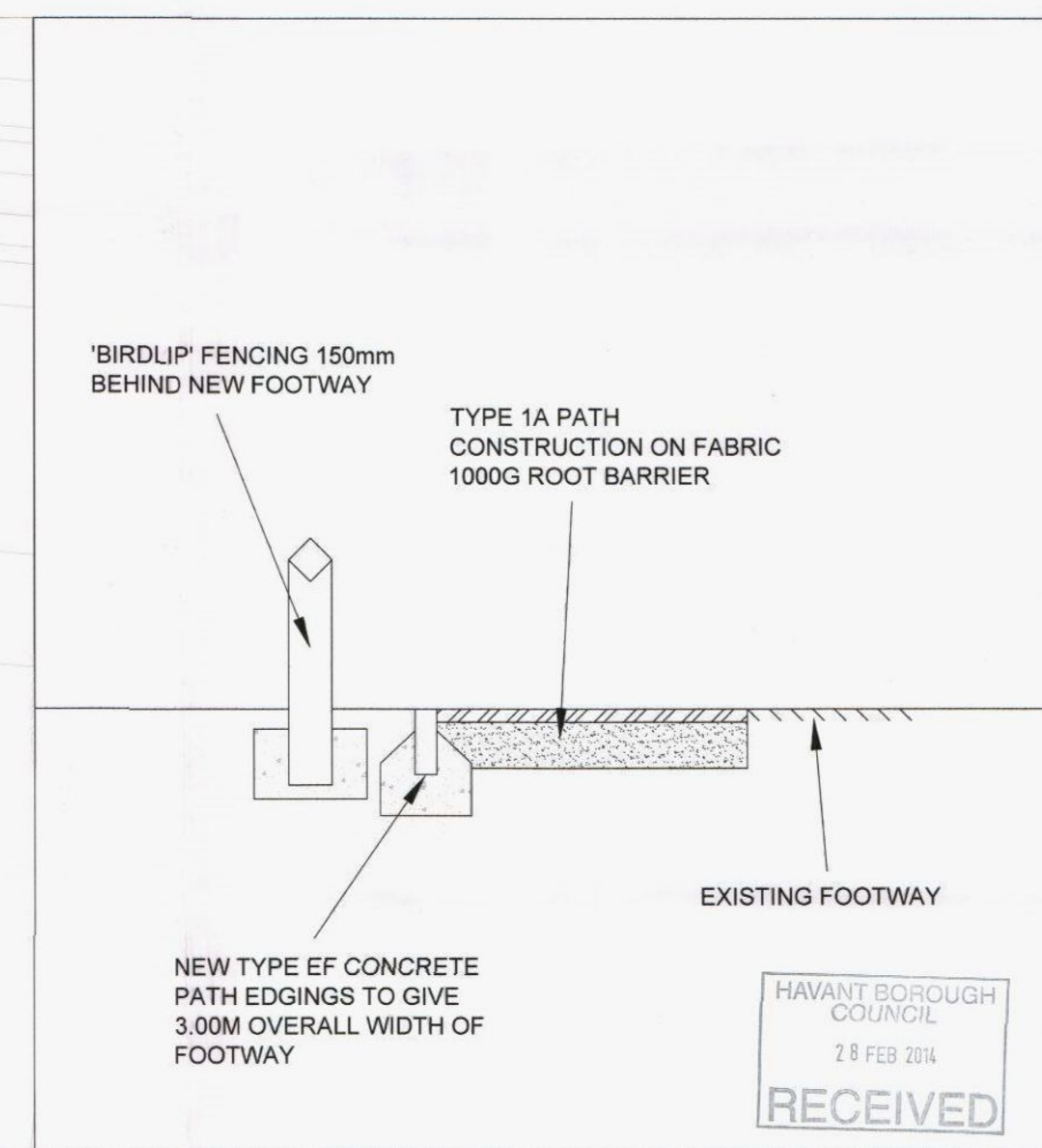
DETAIL OF EXTENDED PATH AND 'BIRDLIP' FENCING NOT TO SCALE
