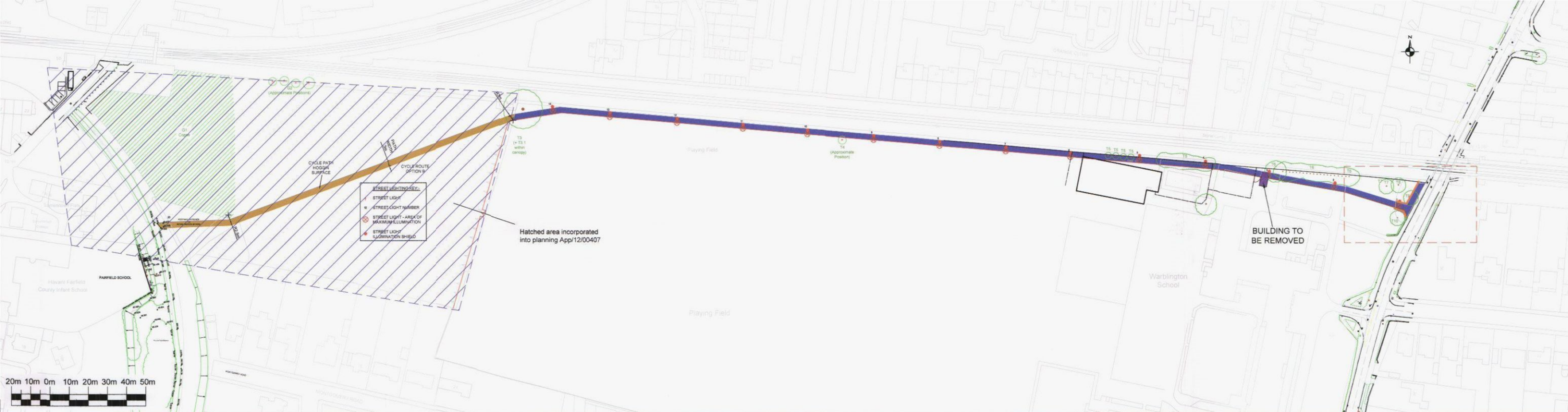
CYCLE PATH LOCATION PLAN SCALE 1:1000
