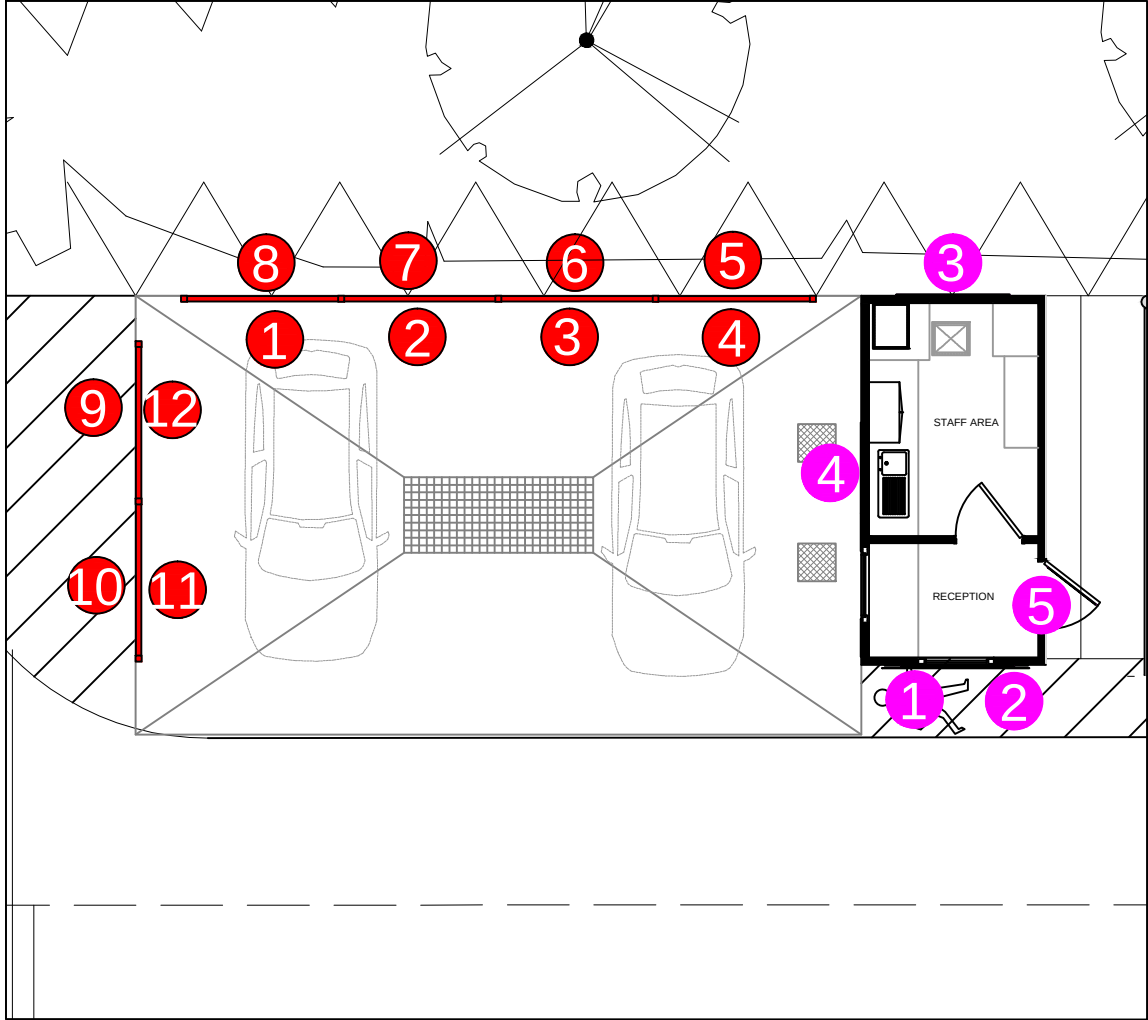
SIGN PLAN 1:100 @ A3
