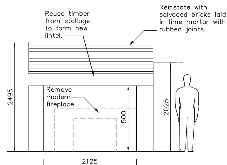
PROPOSED NORTH
