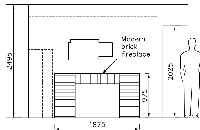
EXISTING NORTH
