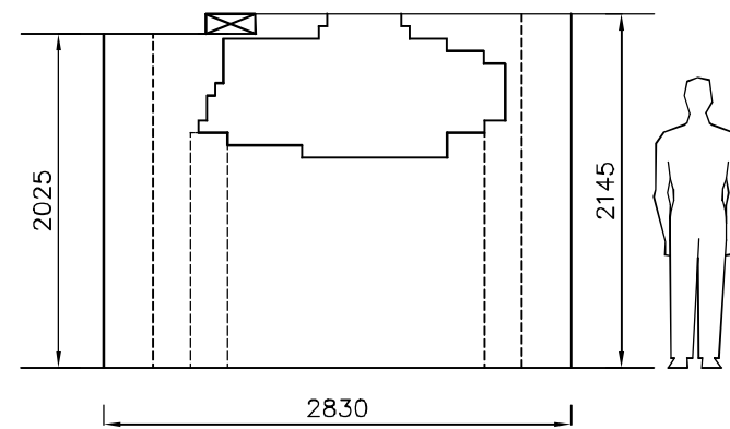
EXISTING SOUTH
