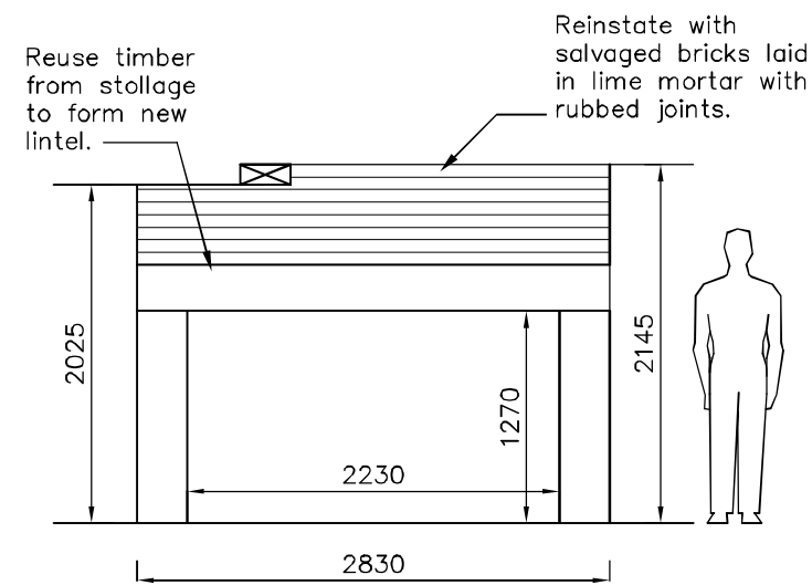
PROPOSED SOUTH
