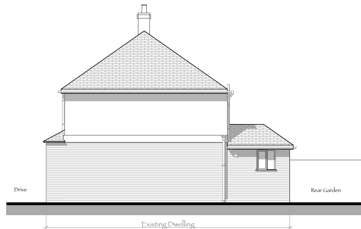
Existing Side Elevation C-C
