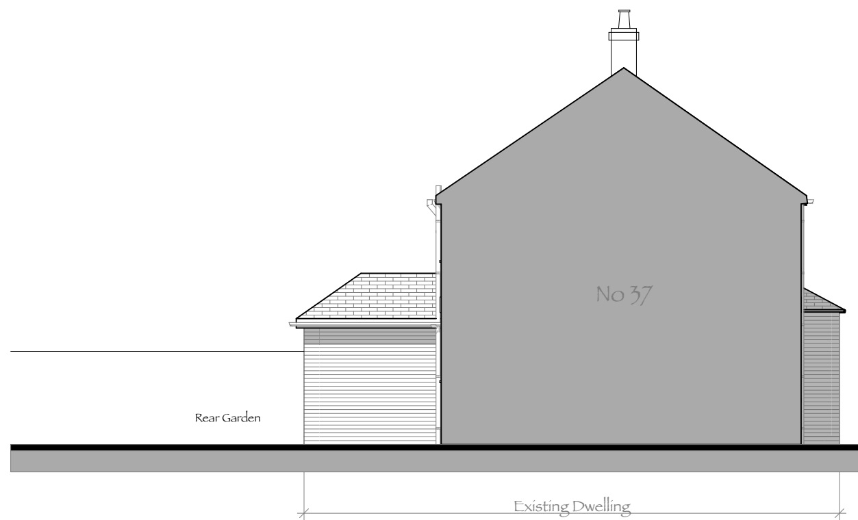
Existing Side Elevation B-B
