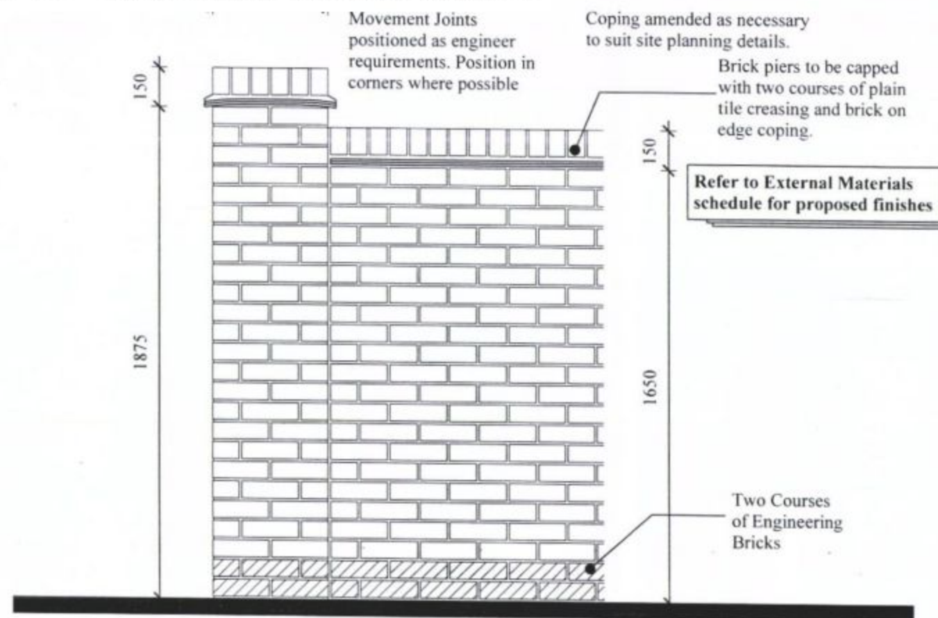
Elevation of Brick Screen Wall
