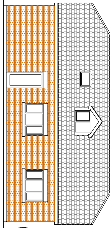
West Elevation PLOT 1
