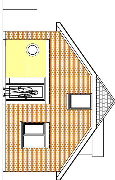
North Elevation
