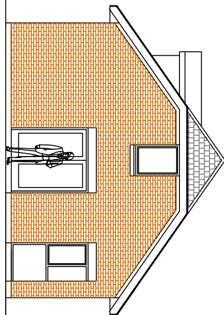
South Elevation
