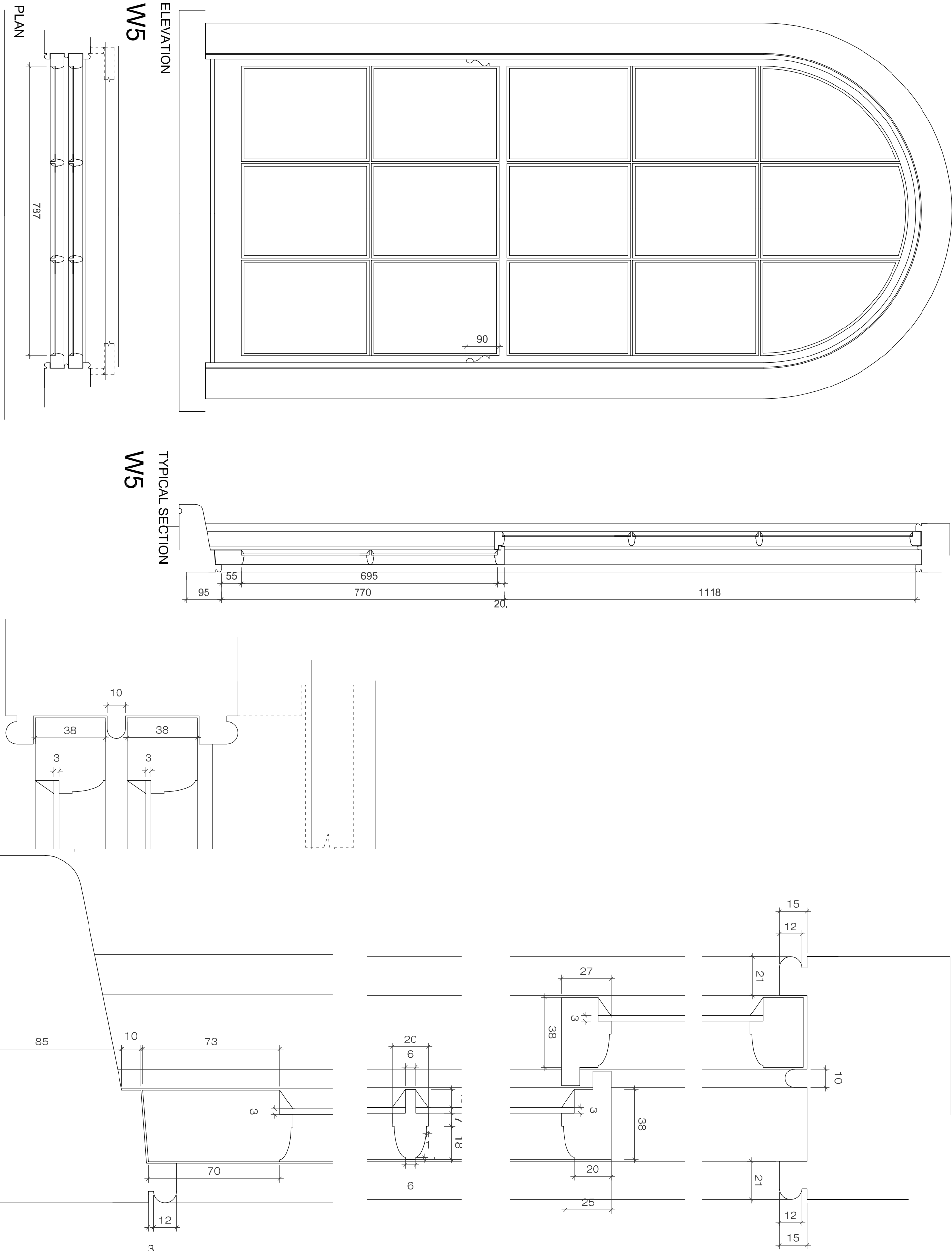
EXISTING - W5 PLANS, ELEVATIONS & TYPICAL SECTION - 1:10
