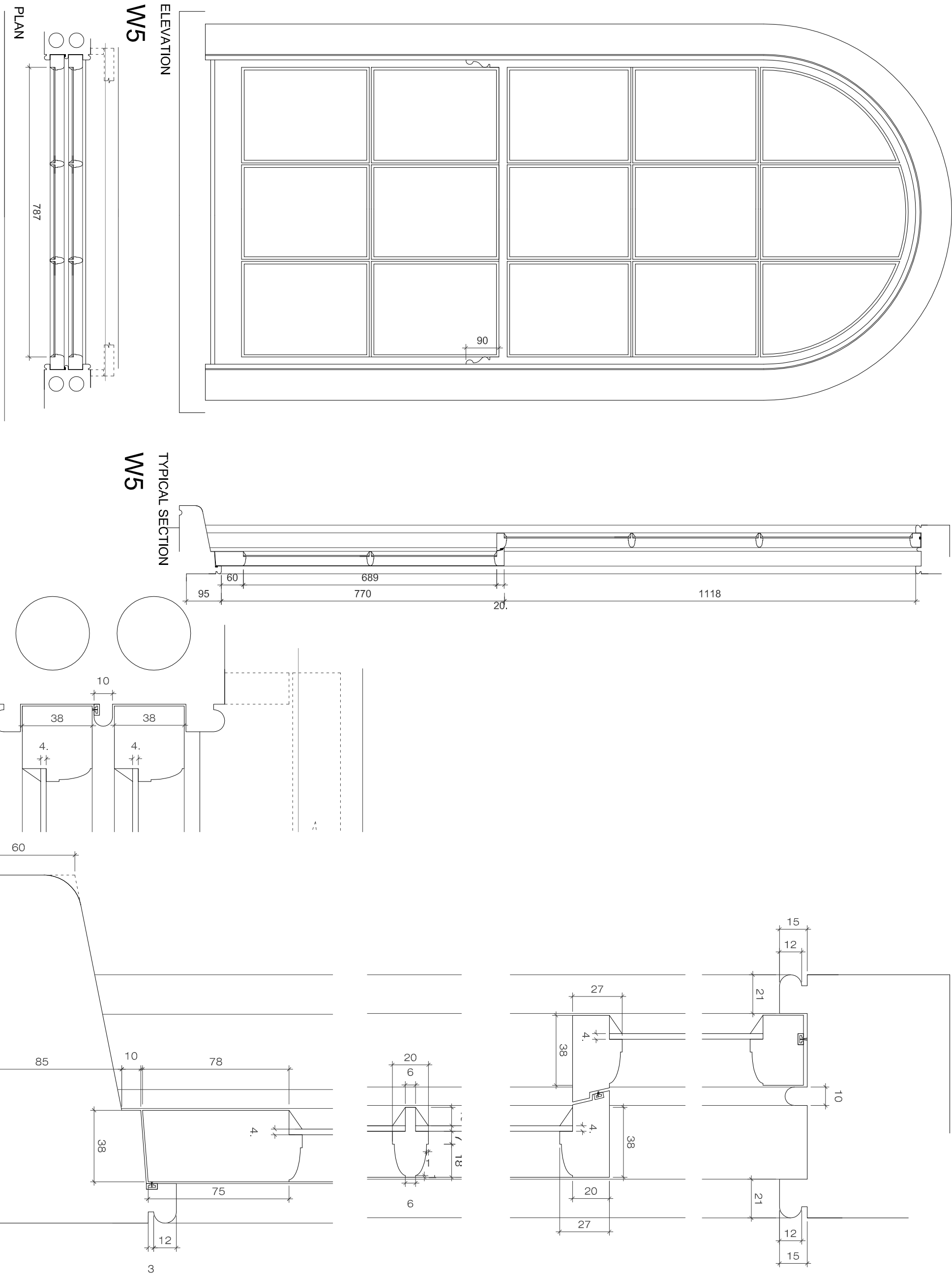
PROPOSED - W5 PLANS, ELEVATIONS & TYPICAL SECTION - 1:10
