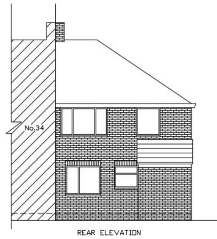
REAR ELEVATION
