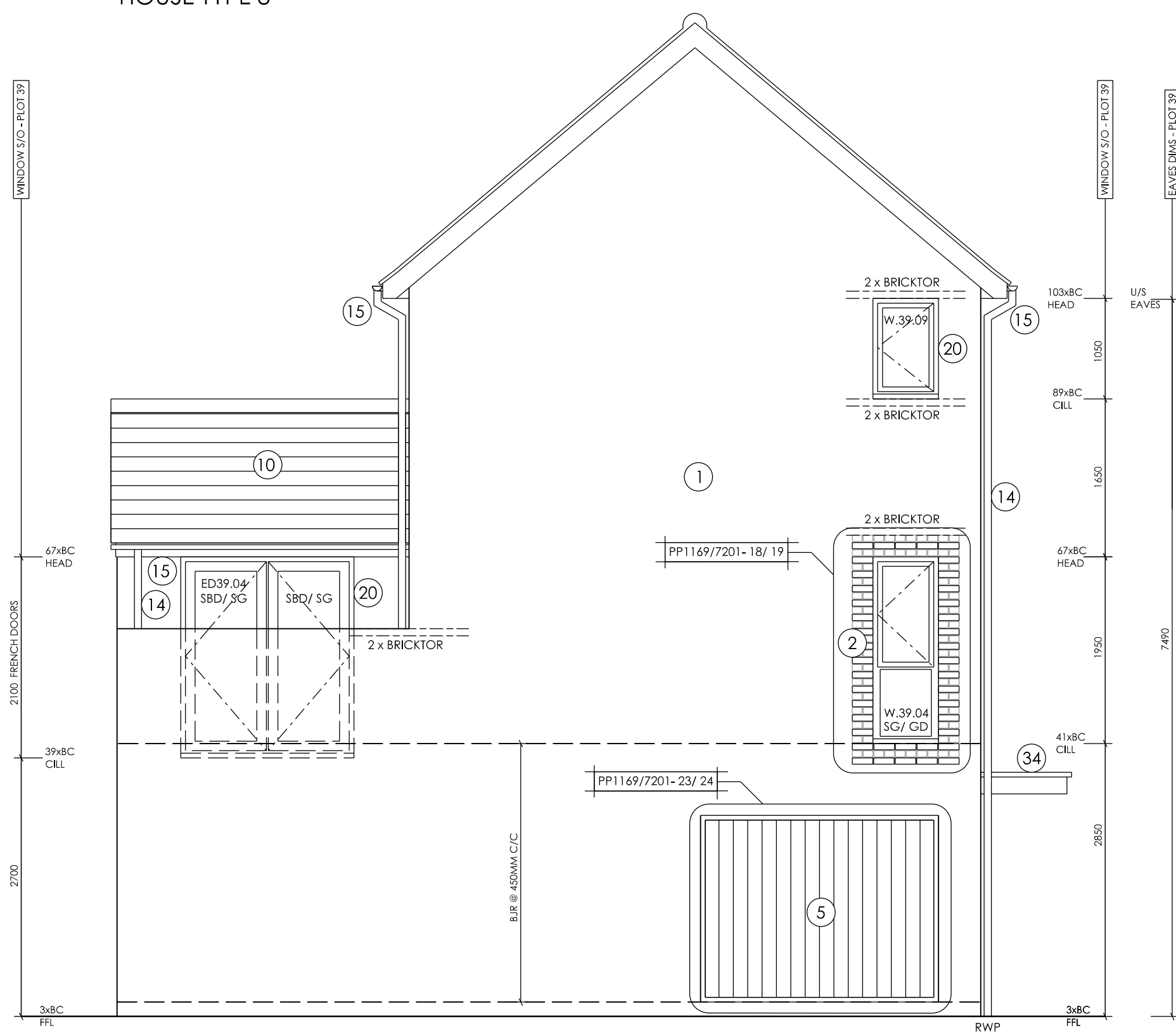
PLOT 40 HOUSE TYPE 8
