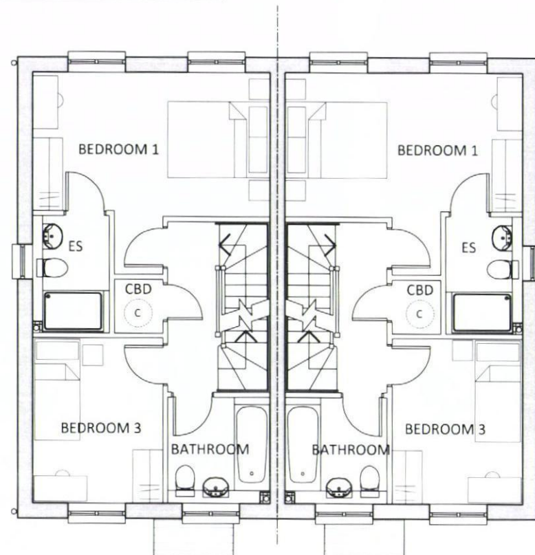
02 37 First Floor Plan GIA - 39.6 sqm per unit
