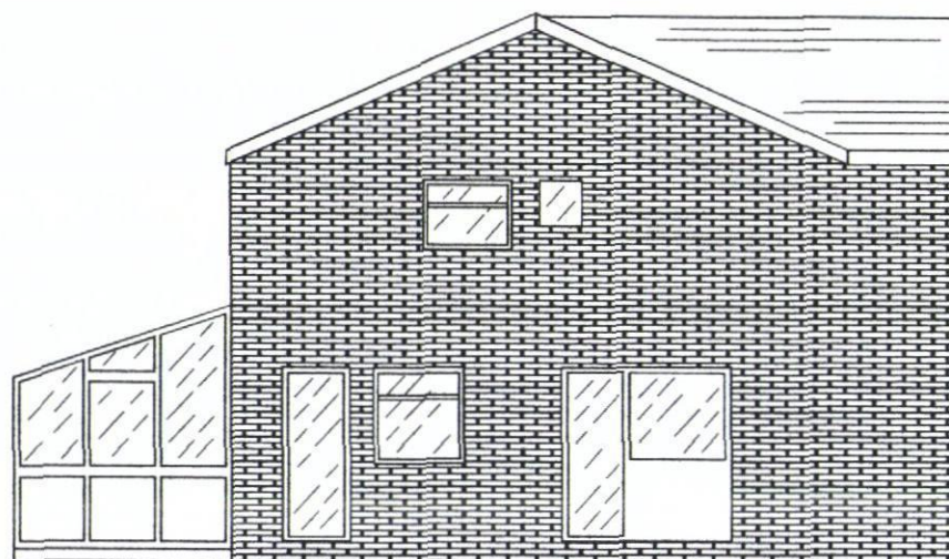
Side elv. west
