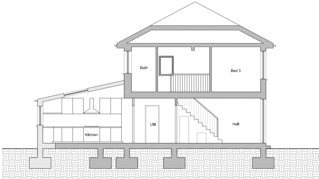
Proposed Section View A-A
