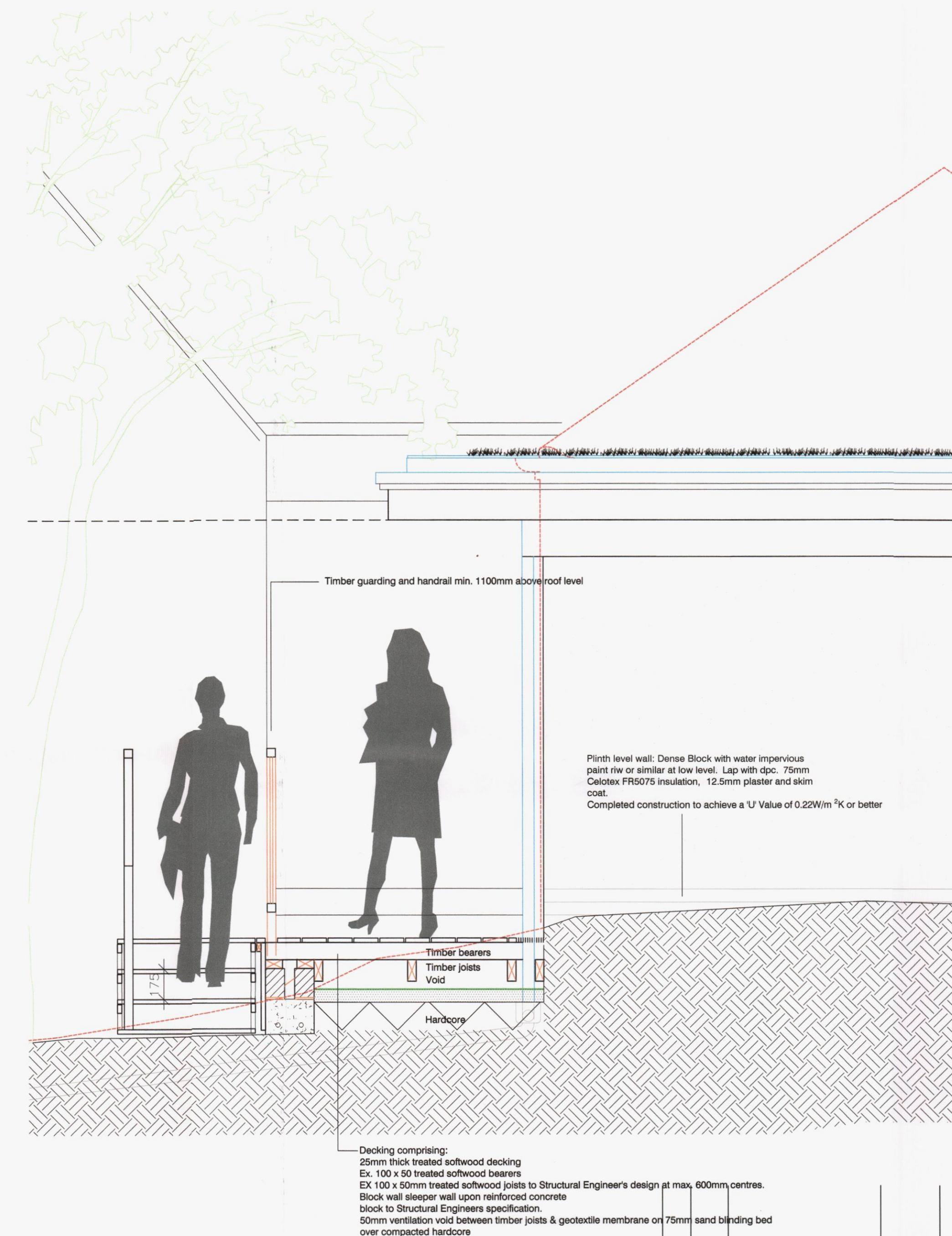
Proposed Section C_C at 1:20
