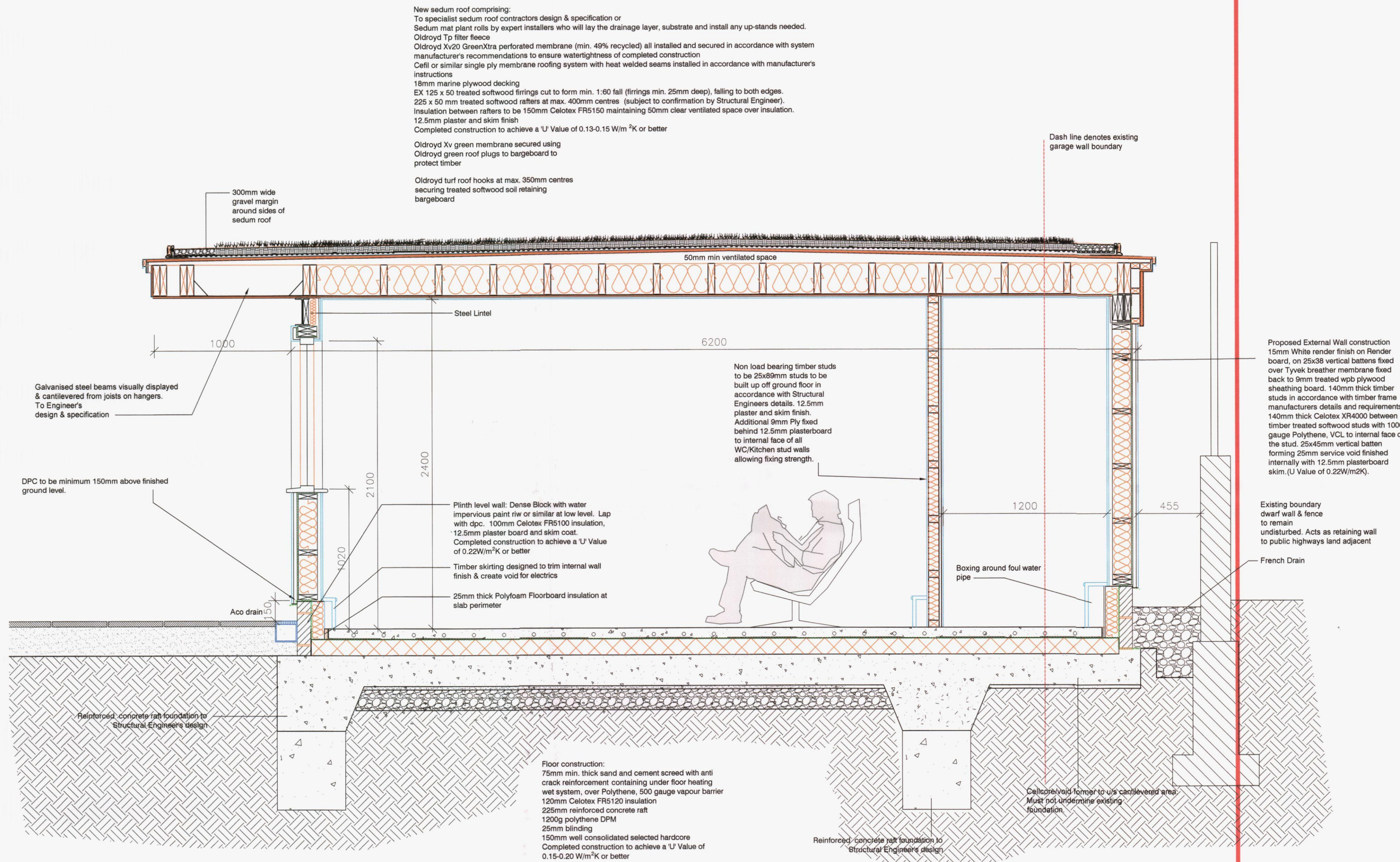
Proposed Section B_B at 1:20
