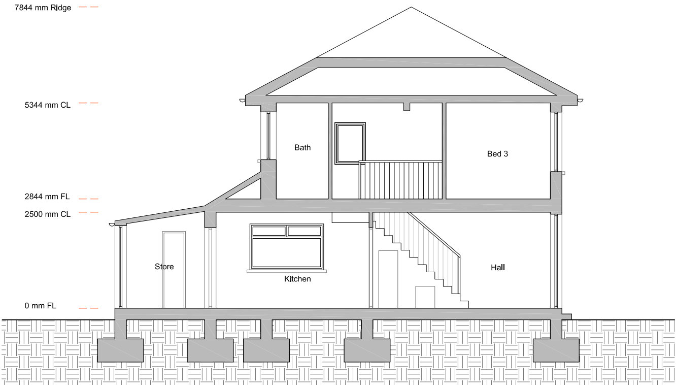
Existing Section View A-A
