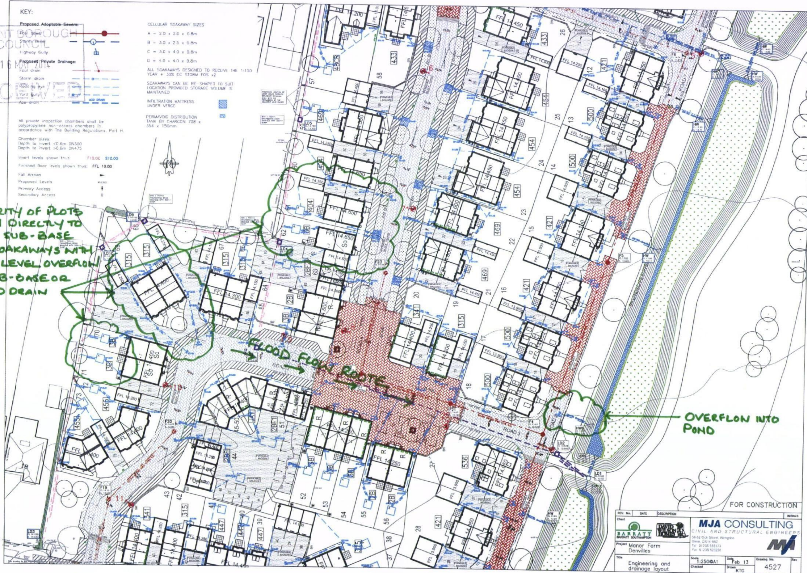
FIG1: EXTRACT OF SURFACE WATER DRAINAGE / OVERFLOWS
