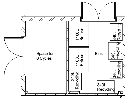
1 Ground 1 : 100
