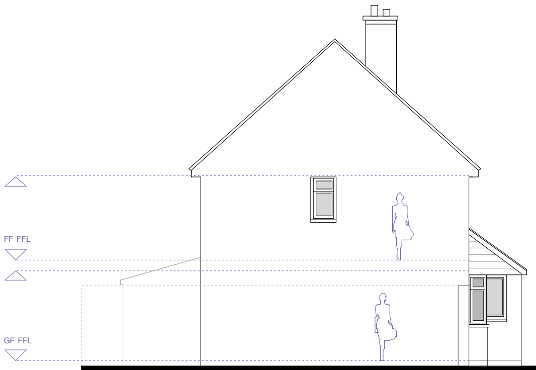
Proposed South East Elevation at 1:100 scale Proposed Section Lines at 1:100 scale
