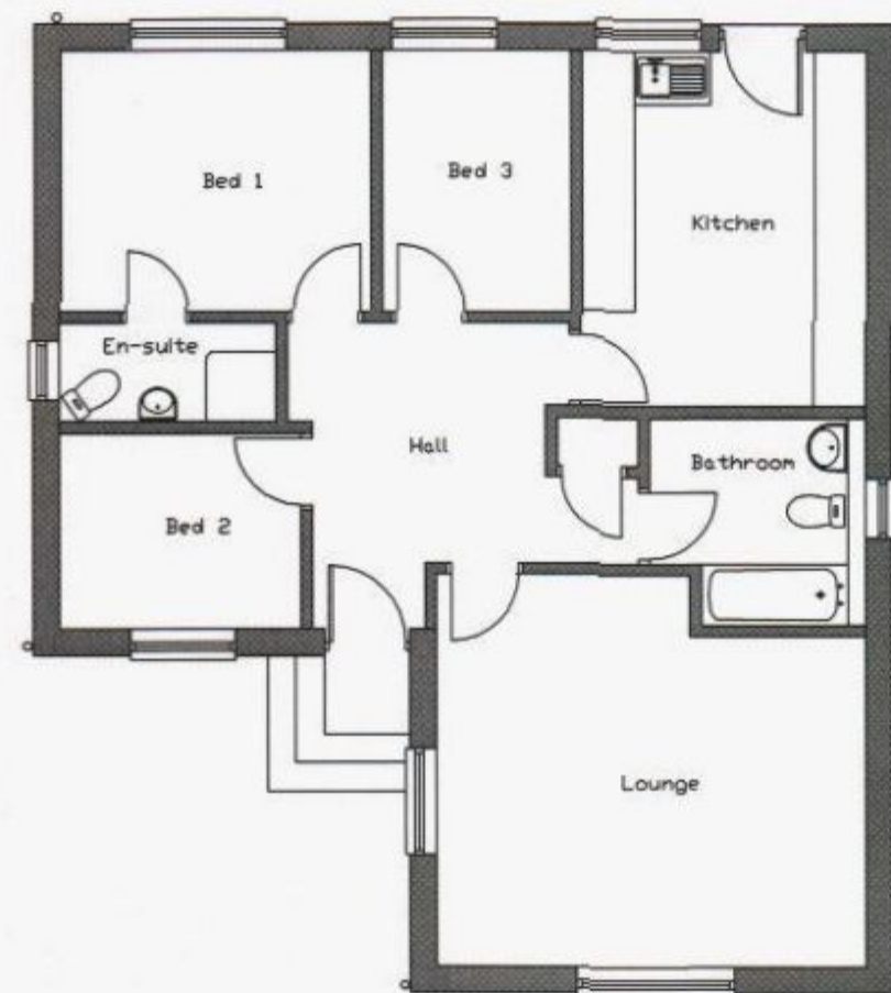
FLOOR PLAN
