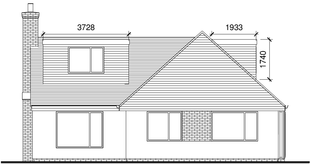
Volumetrics East Elevation 1 : 100
