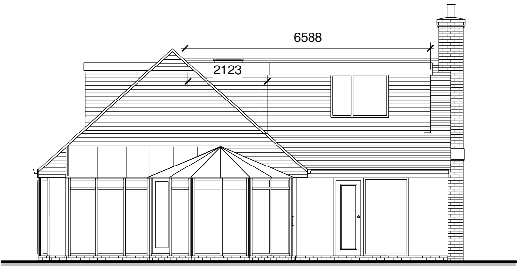
Volumetrics West Elevation 1 : 100
