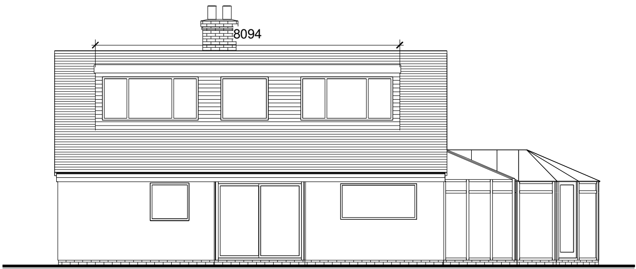
Volumetrics North Elevation 1 : 100
