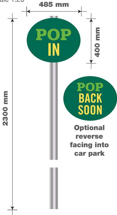
ITEM 13 (Qty 2) Aluminium panel with applied vinyl text. Fixed to 78mm dia. post. Non illuminated. Scale 1:20
