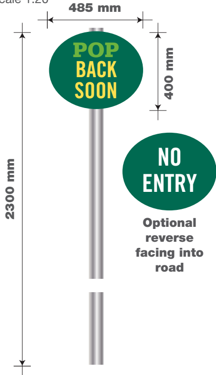
ITEM 13A (Qty 2) Aluminium panel with applied vinyl text. Fixed to 78mm dia. post. Non illuminated. Scale 1:20
