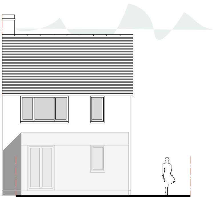
Existing West Elevation at 1:00 scale
