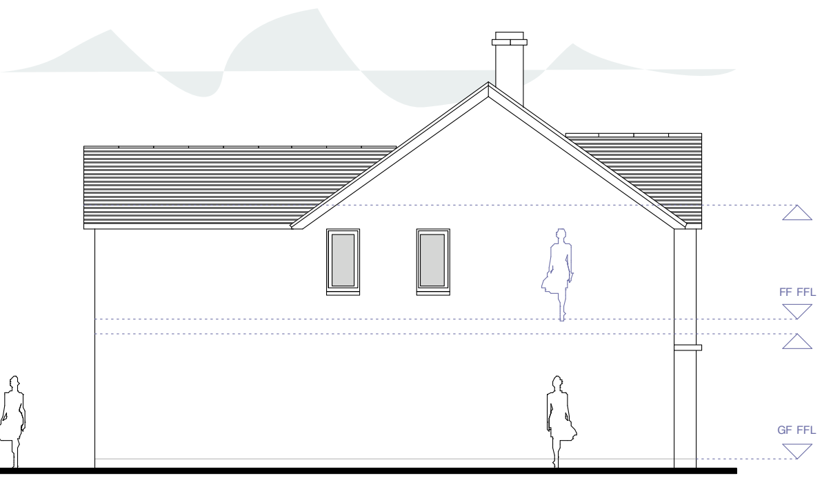
Proposed South Elevation (Section) at 1:00 scale
