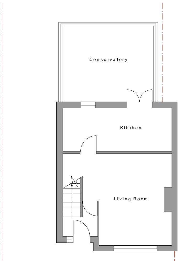
Existing GF Plan at 1:00 scale
