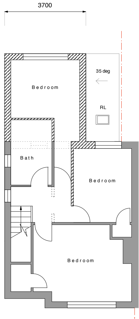
Proposed FF Plan at 1:00 scale
