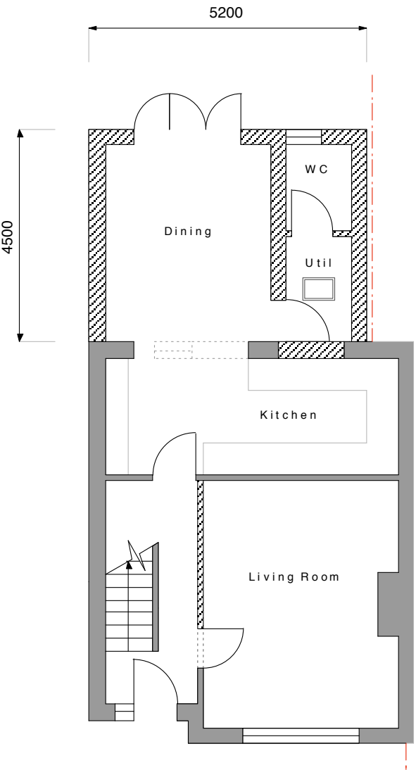
Proposed GF Plan at 1:00 scale
