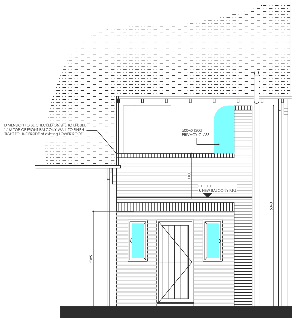
NORTH EAST ELEVATION 1:50
