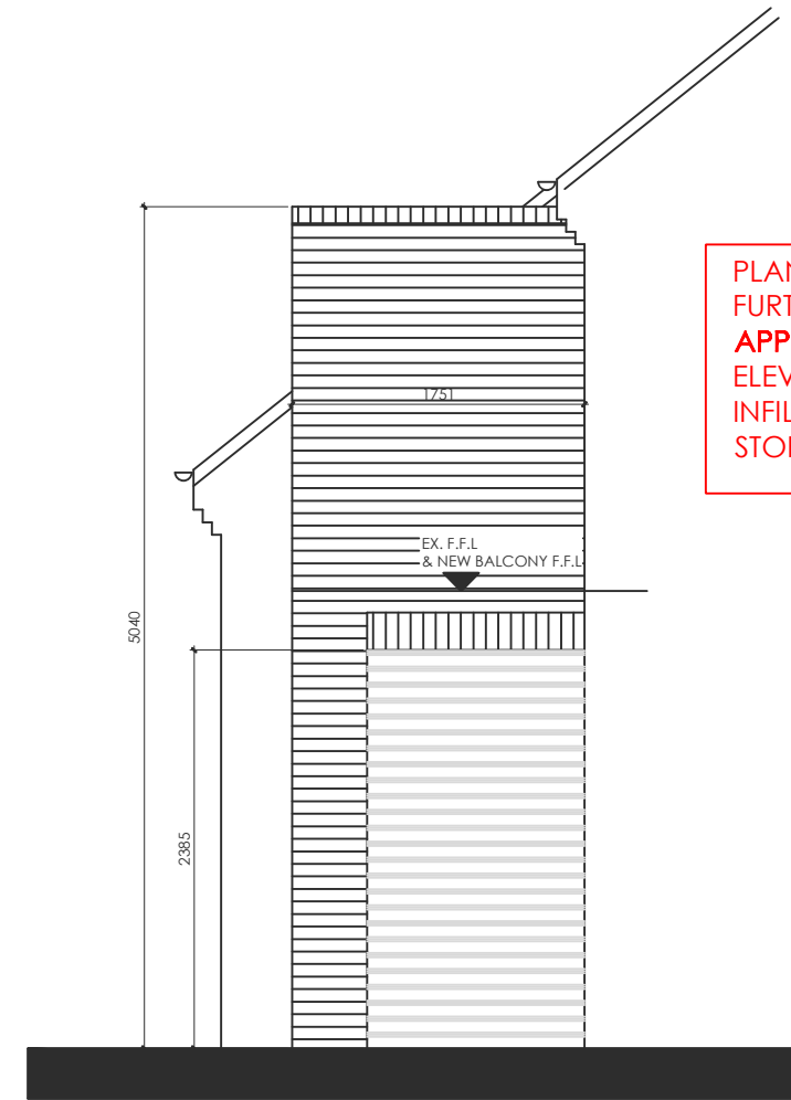
NORTH WEST ELEVATION 1:50
