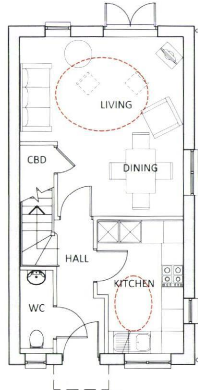
01 25 Ground Floor Plan GIA 38sqm
