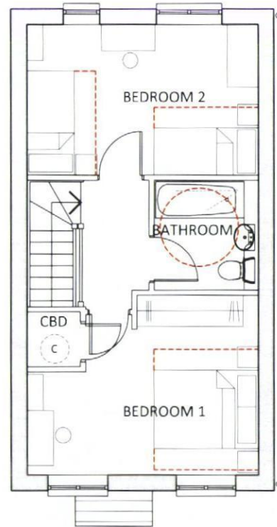
02 25 First Floor Plan GIA 38sqm
