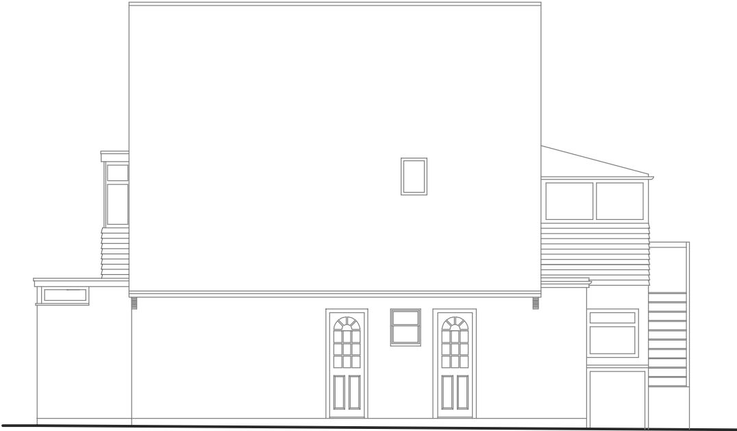
WEST ELEVATION
