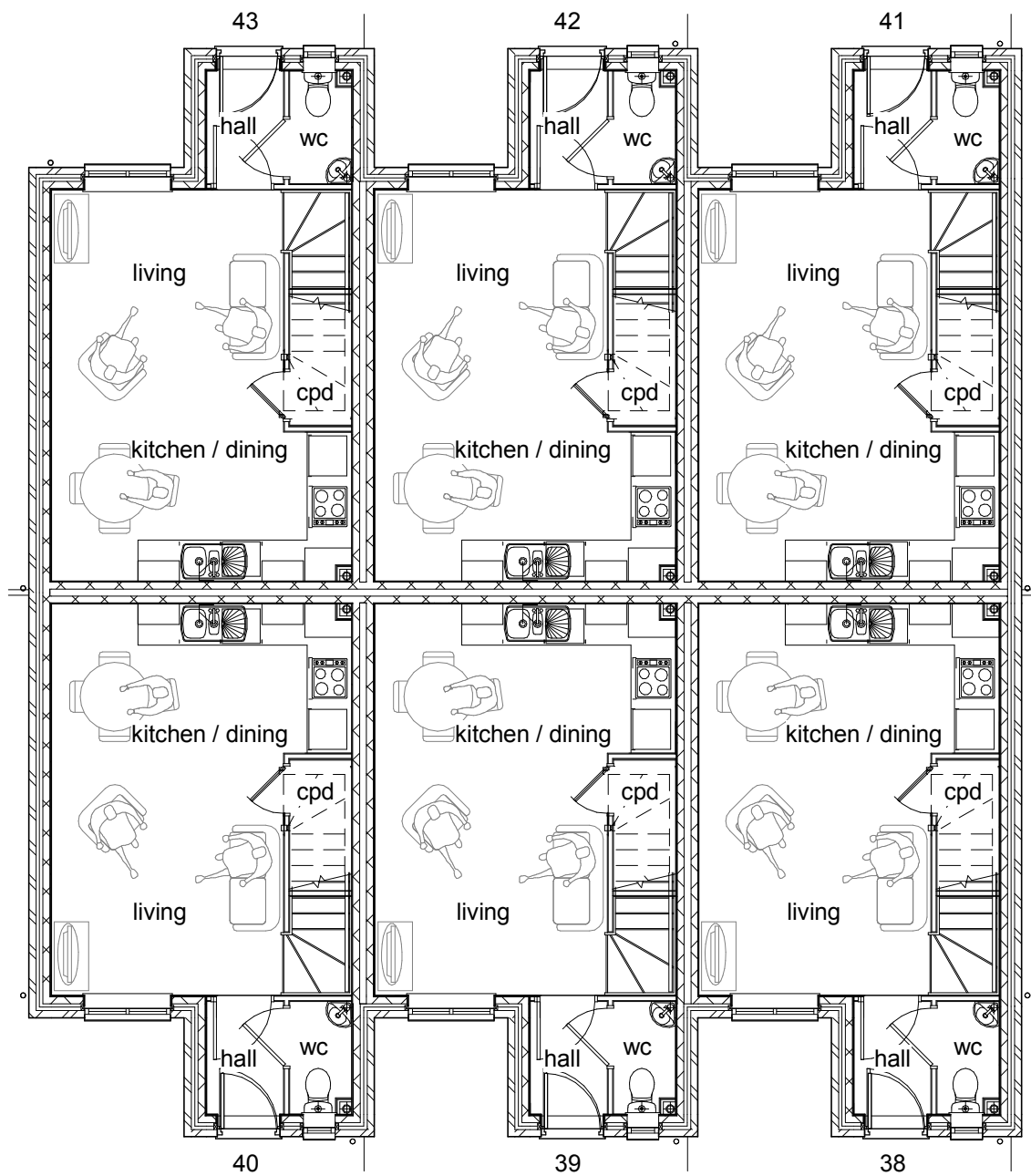
1 Ground Floor 1 : 100
