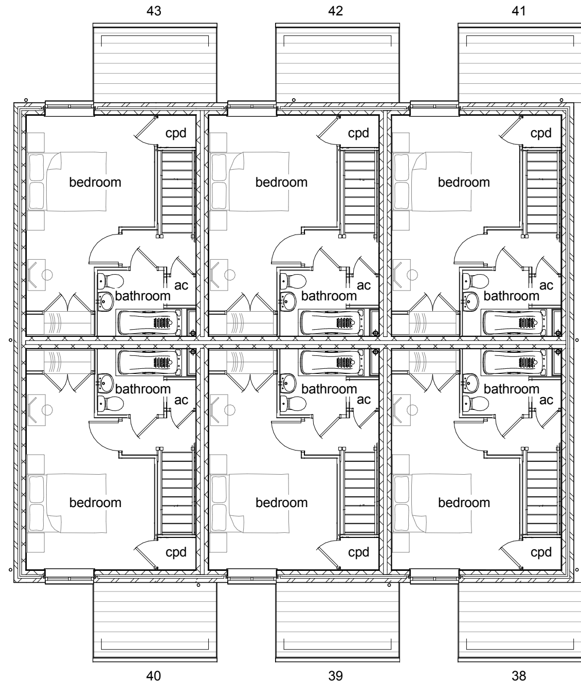
2 First Floor 1 : 100
