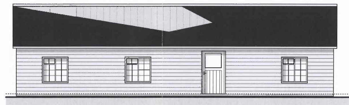
South Elevation
