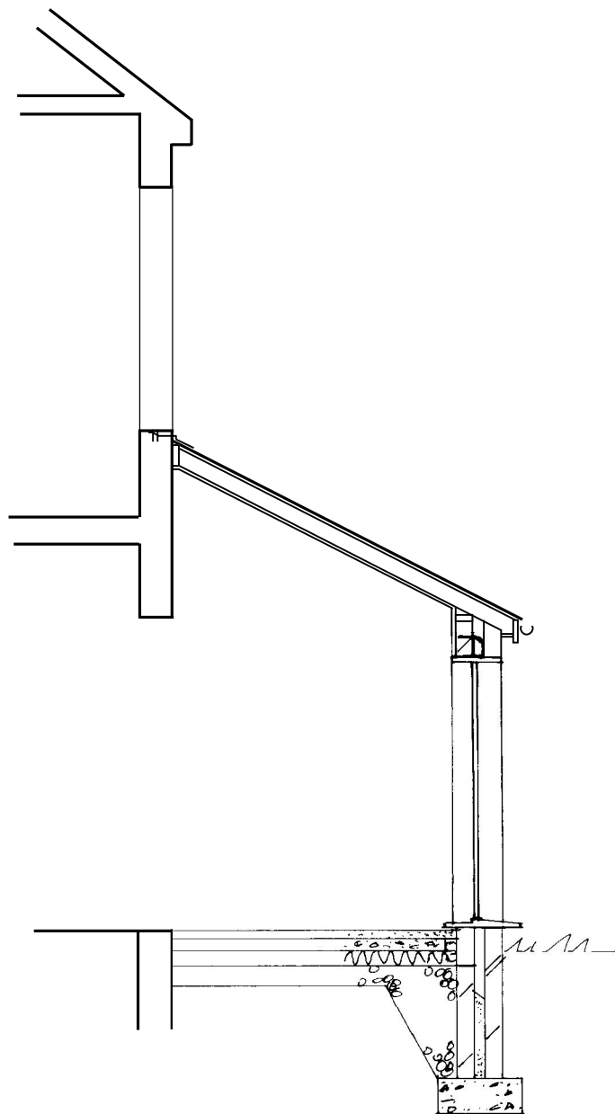
Section Thro Rear Extn
