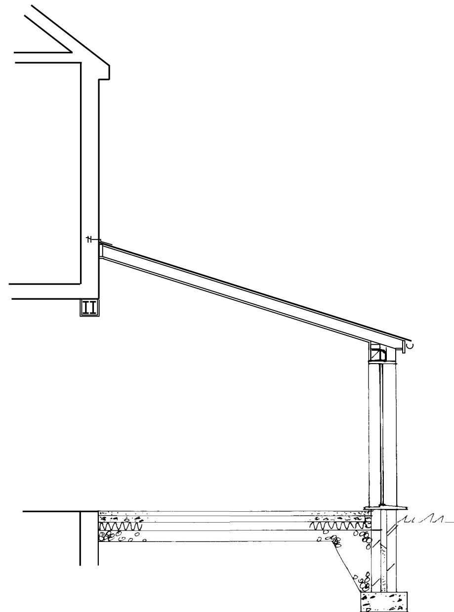
Section Thro Side Extn
