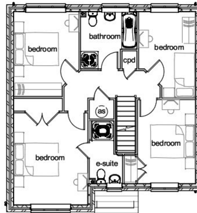
2 First Floor
