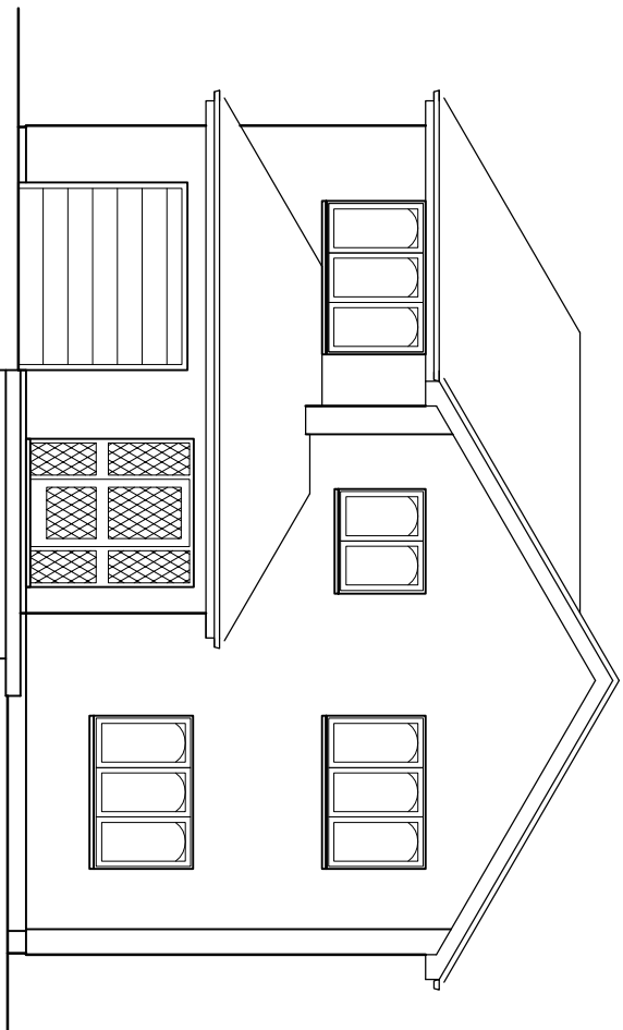
Front elevation: EXISTING 1:100
