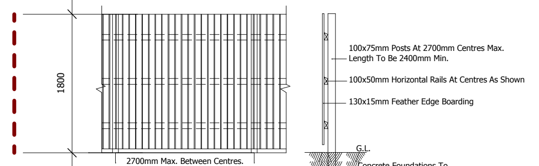
1.8m High Close Boarded Fence
