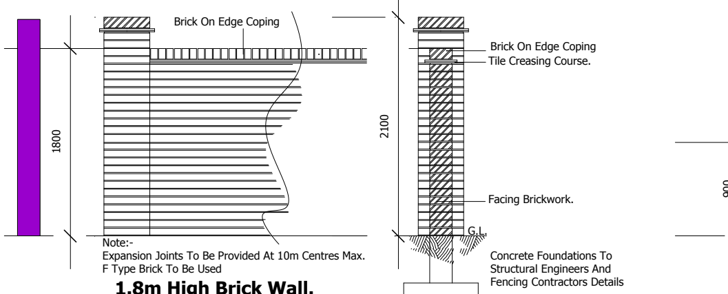
1.8m High Brick Wall.
