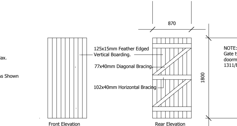
1.8m High Timber Close Boarded Gate.
