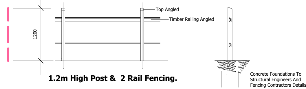
1.2m High Post & 2 Rail Fencing.
