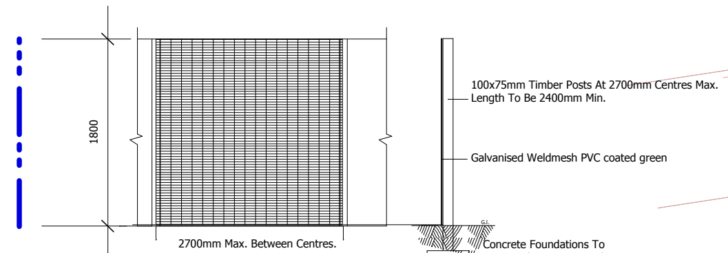
1.8m Galvanised Weldmesh pvc Green
