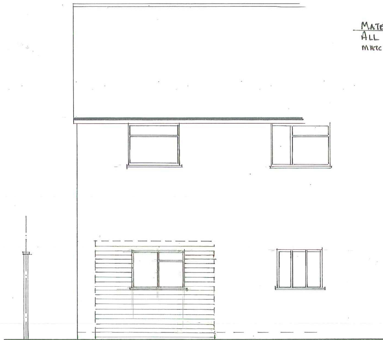
SOUTH ELEVATION.
