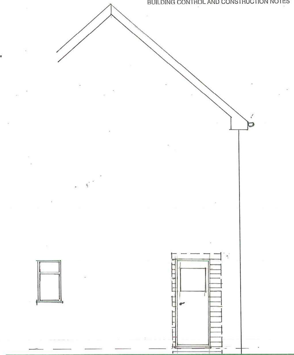
WEST ELEVATION.
