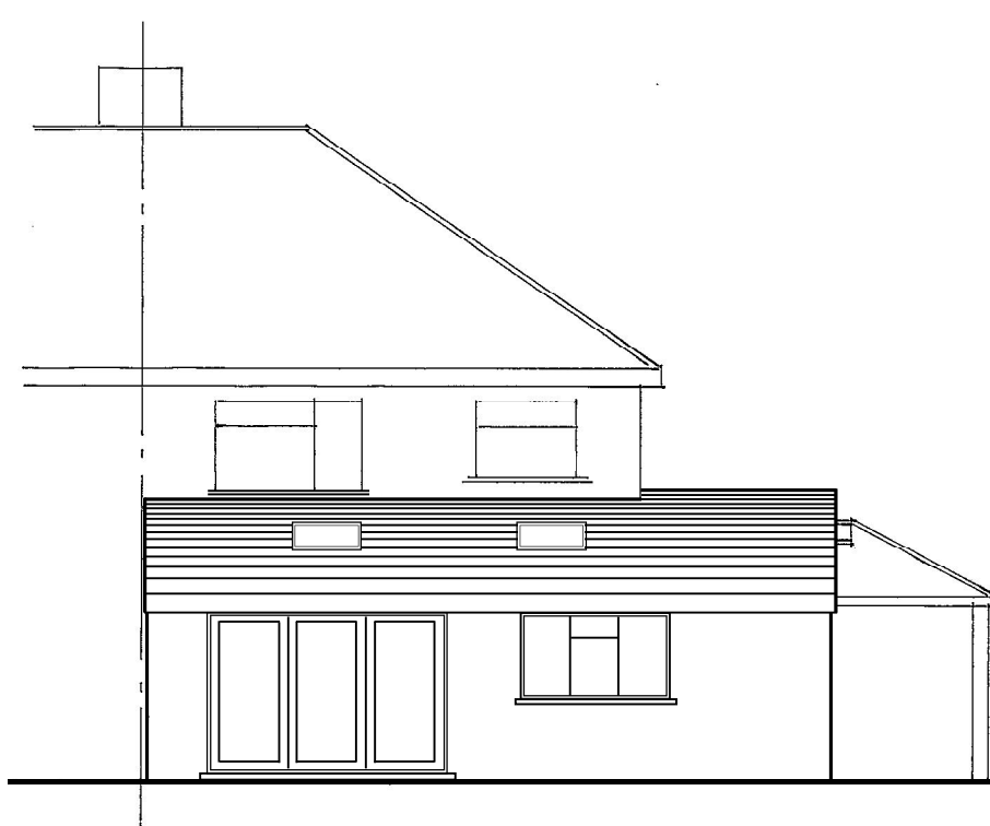
Proposed NW/Rear Elevation
