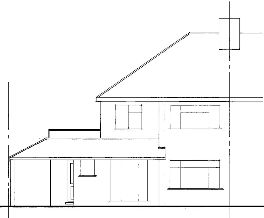
Proposed SE/Front Elevation
