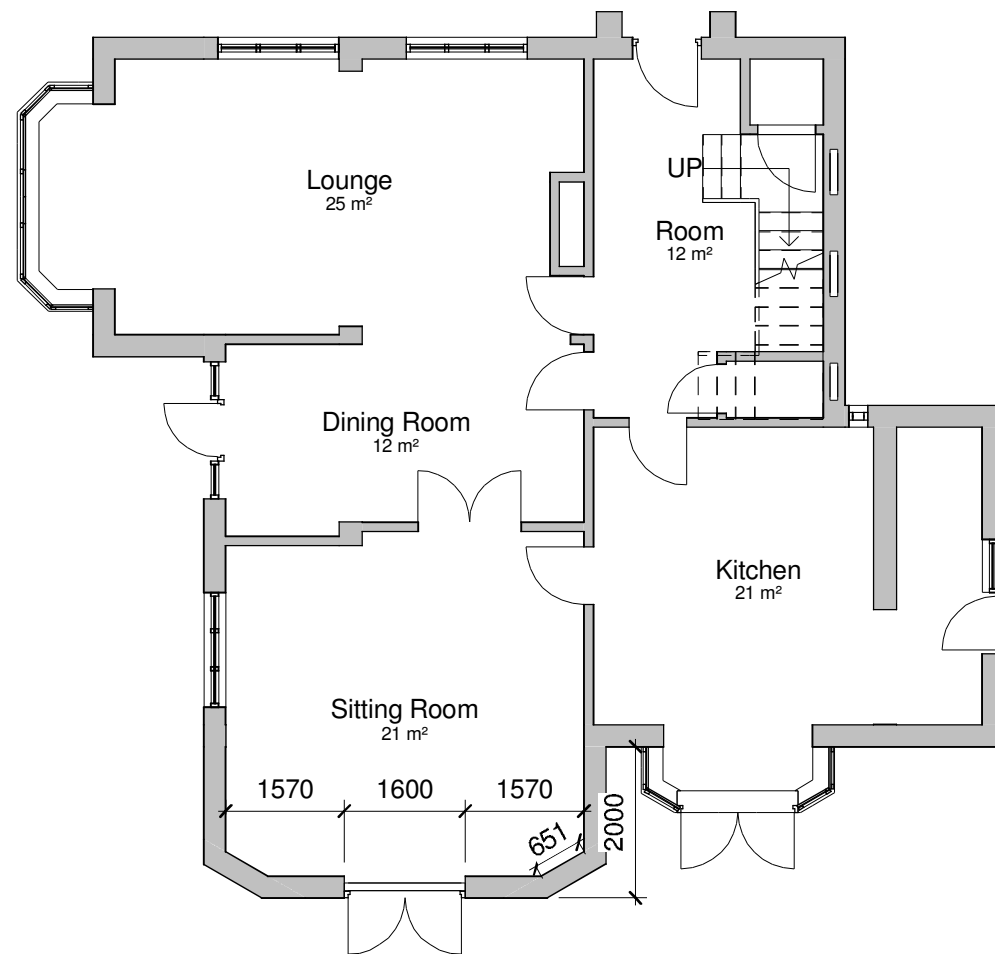
Proposed Ground Floor 1 : 100
