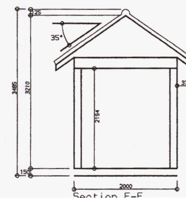
Section E-E
