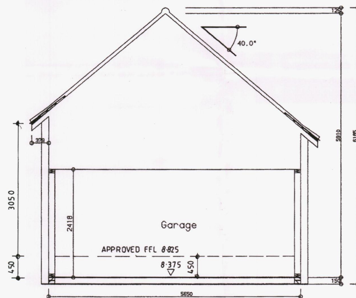
Section C-C
