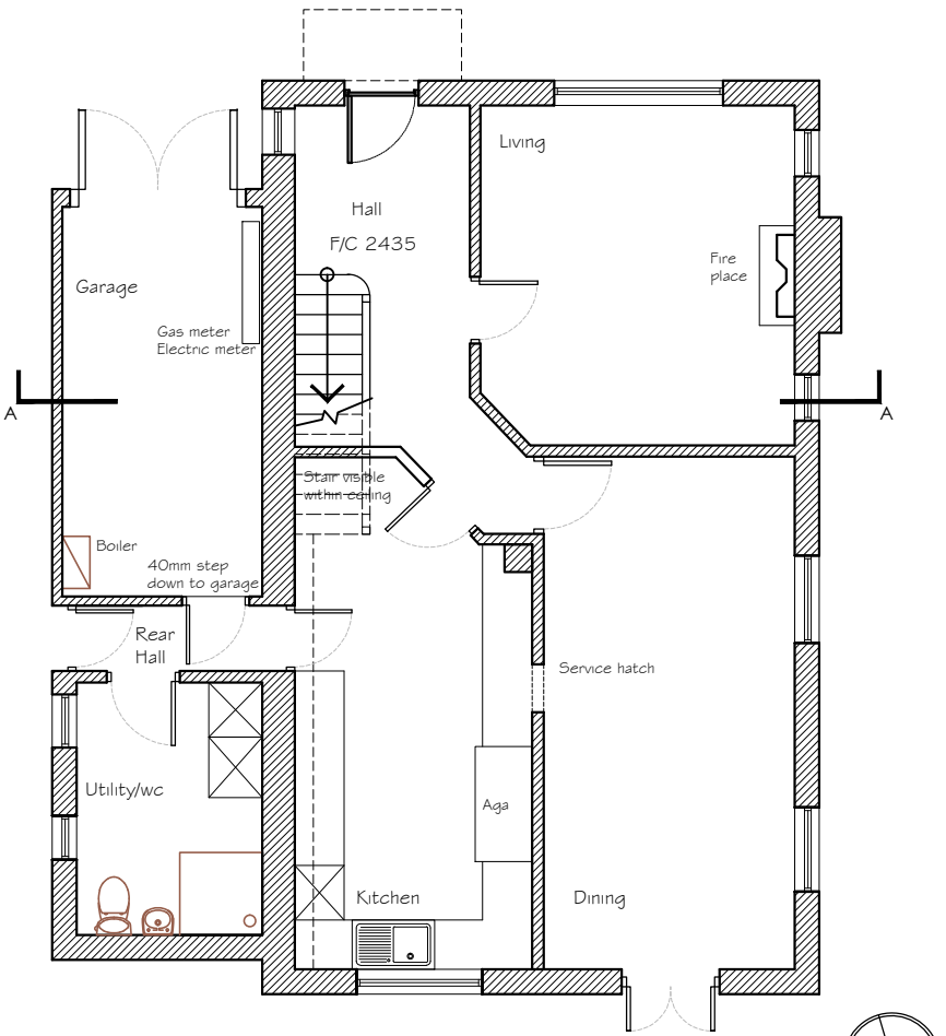
GROUND Floor Plan Plans 1:100 @ A1 1 0 1 2 3 4 5 6 7 8 9m 1:100
