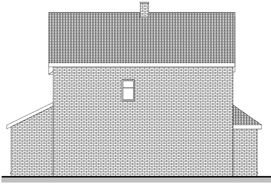
Existing LHS Elevation 1 : 100
