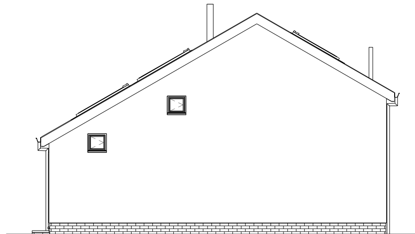
WEST ELEVATION
