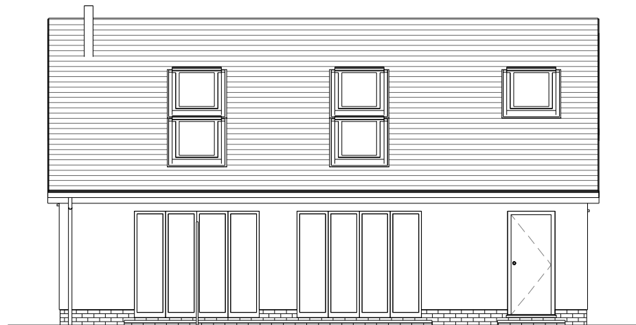
NORTH ELEVATION
